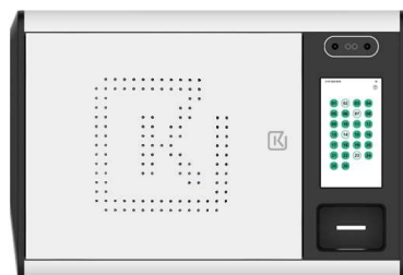
Android Terminal
